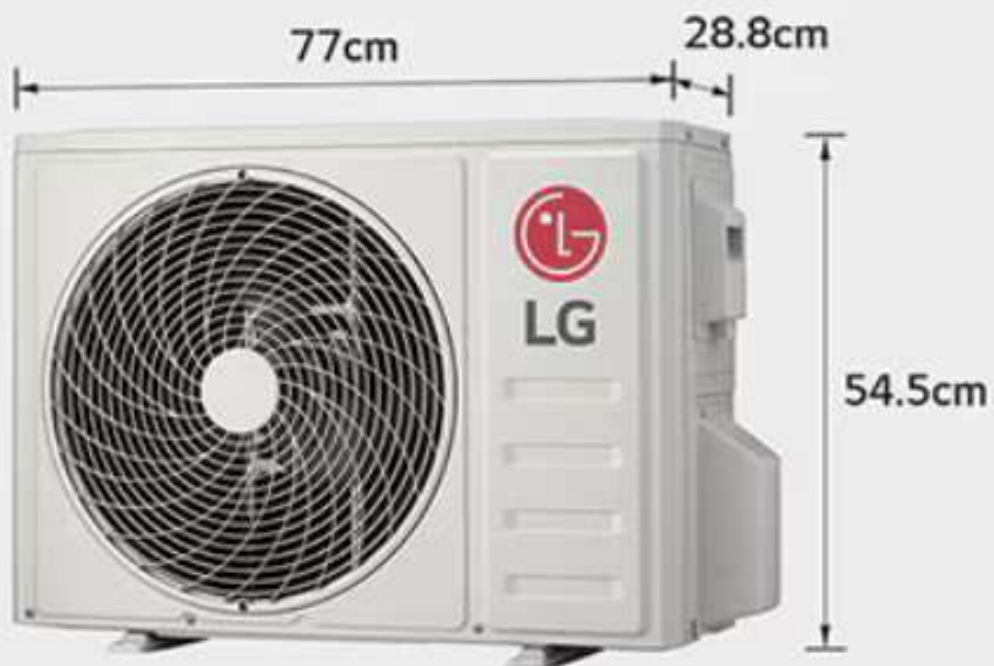
Outdoor Unit
