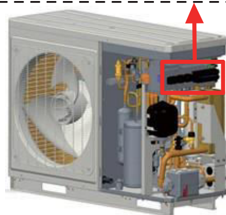
Terminal blockXT5
