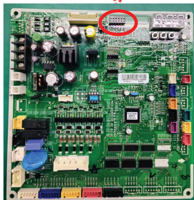
DIP_SW01D
